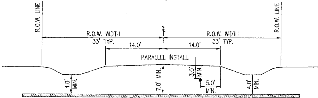
ROADWAY CROSS SECTION NO SCALE
